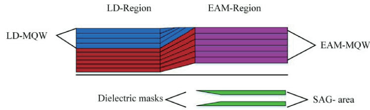
Figure 1 (Color online) Schematic material structure of an EML fabricated using our novel process.
