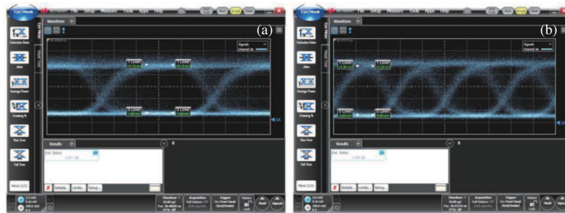
Figure 3 (Color online) Eye diagrams of an EML at 10 Gb/s (a) and 20 Gb/s (b) modulations in BTB configuration [16] ©Copyright 2018 IEEE.
